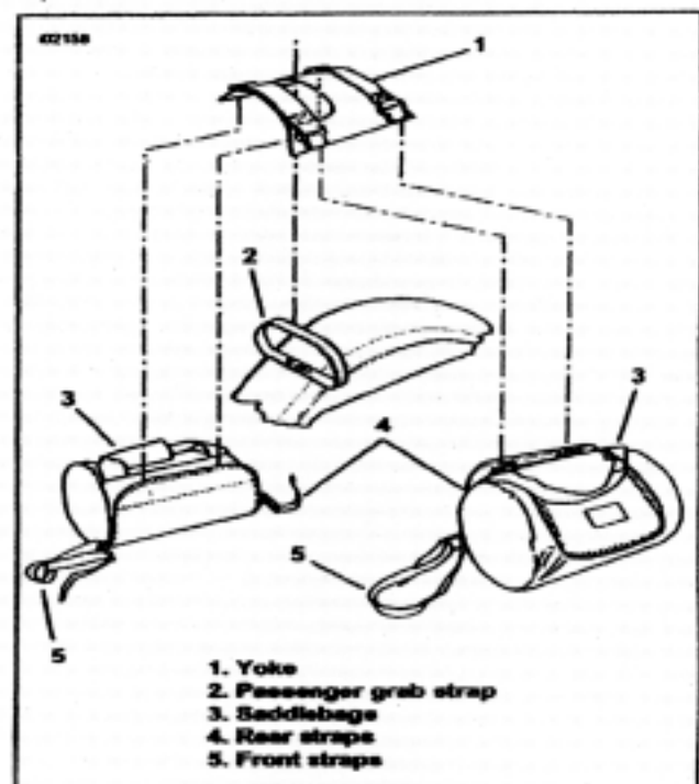
Figure 1. Install Saddlebags
